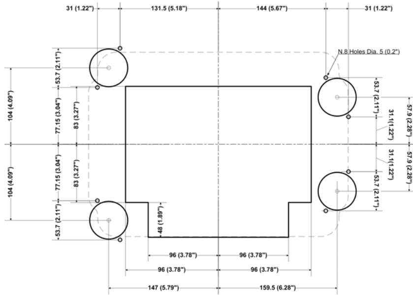
Dimensions in millimetres and (inches)
